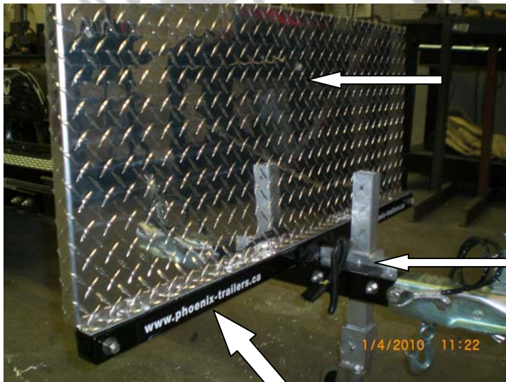
Optional rock guard installed using (4) 7/16" bolts at the bottom and (1) 7/16" bolt at the wheel chock.
